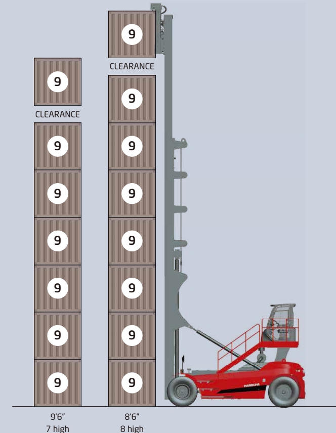
H90EC-8
